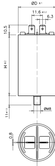
Execution for D= Ø36+50
